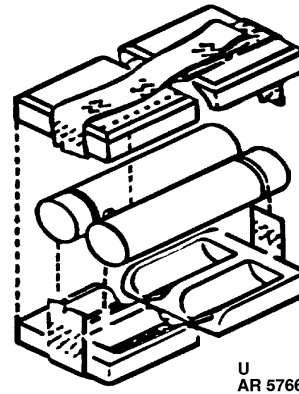
Figure 3-11.1. Grenade/spacer assembly
